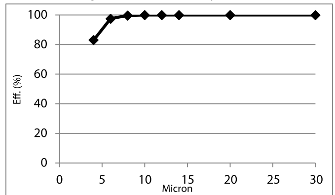
Average Filtration Efficiency (ISO 16889)
