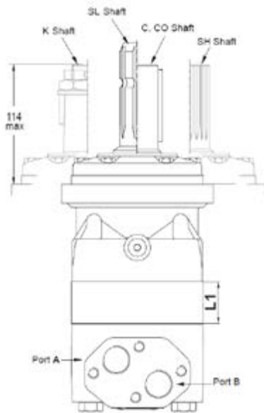
- Standard Mount SAE 4-bolt
