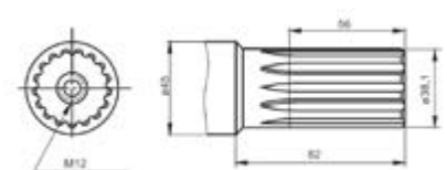
SH 1.1/2" 17T Splined Shaft
