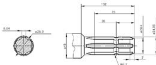
SL 1.3/8" 6T Splined PTO Shaft
