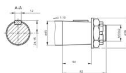
K 45mm 1:10 Tapered Shaft
