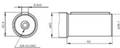
CO 1.1/2" Straight Keyed Shaft
