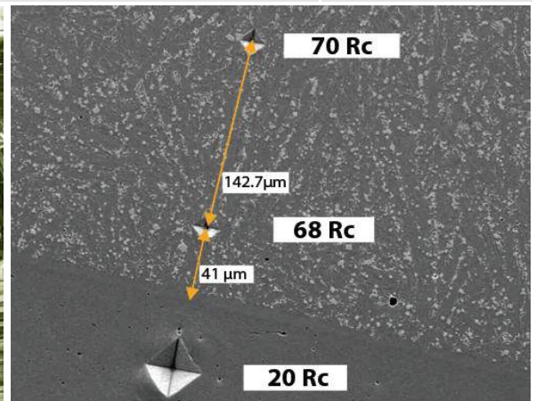
Low dilution, predictable wear rates. Properties and hardness remain consistent throughout the entire hard facing layer.
