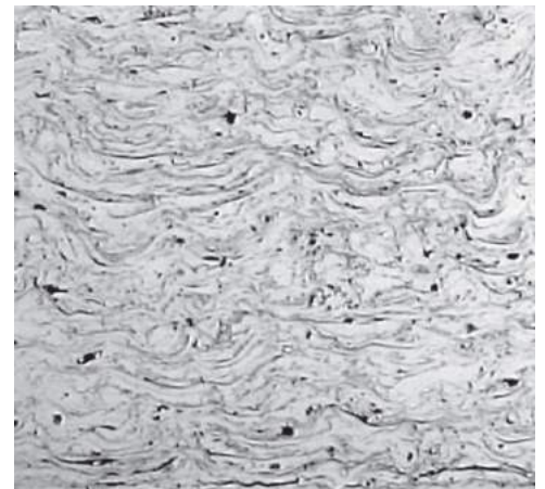
Structure of cold arc sprayed coating
