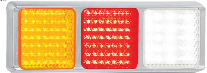
Chrome Bracket - Stop/Tail/Indicator/Reverse 100CARWM - Blister, 12-24 Volt
