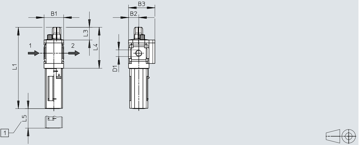
[1] Installation dimension
