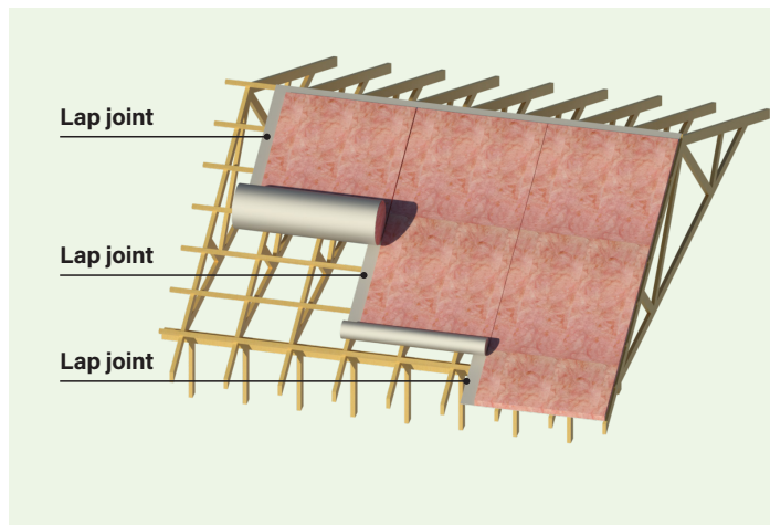
Figure 1: Vertical installation
