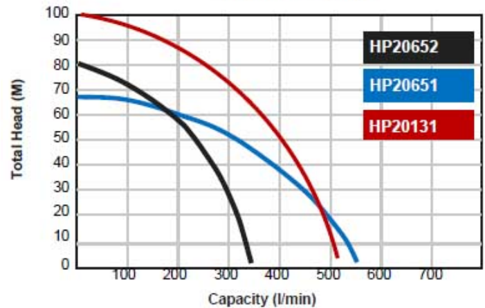
Performance Curve
