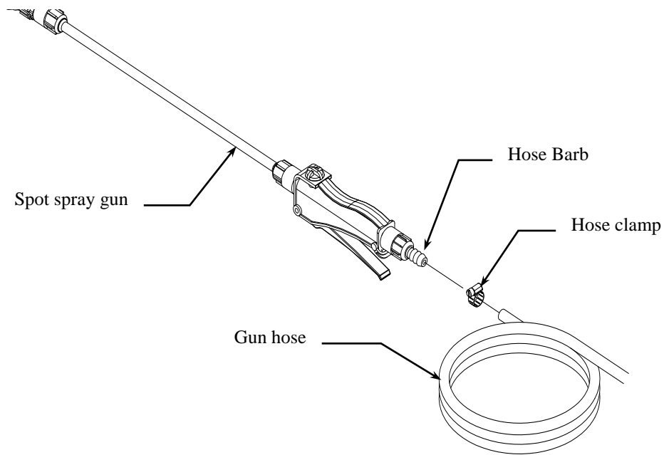
K16000-2 Hose Clamp Qty 1
