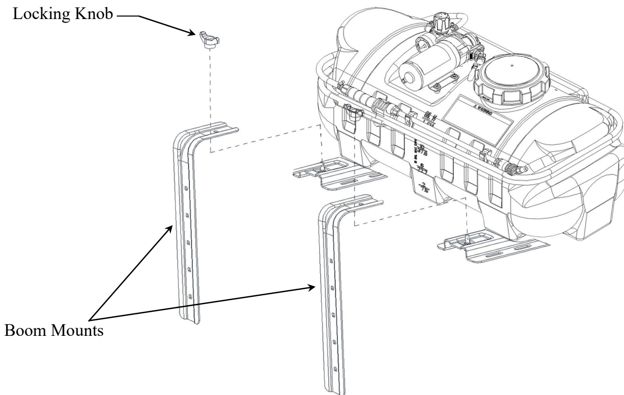
Boom Mount K16-798537 (Qty 2)
